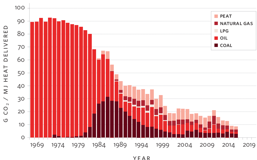
SPECIFIC CO 2 EMISSIONS FROM SWEDISH DISTRICT HEATING BETWEEN 1969 AND 2015 BY INPUT FUEL
